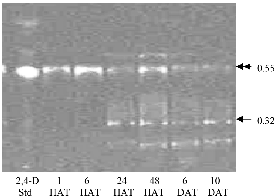
Figure 1. Thin layer chromatography of extract from the treated soybean leaflet. Bright spots indicate the presence of ^{14}\text{C} . Each lane is labeled with the time after application, Std is Standard 2,4-D, HAT is hours after treatment and DAT is days after treatment. The Rf values are 0.55 for the 2,4-D standard and 0.32 for the metabolite.
